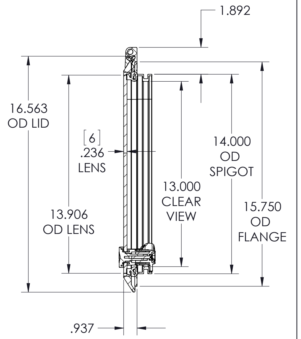
SECTION B-B
